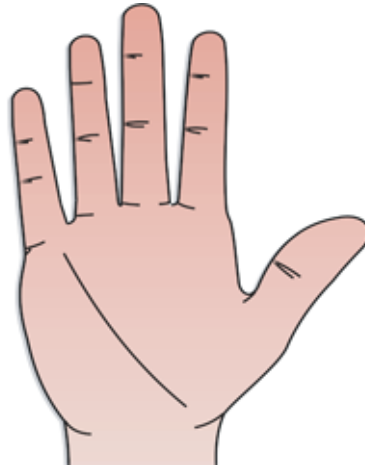
Mercury-Fifth
