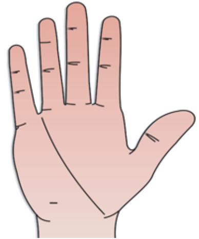
Venus-Fifth
