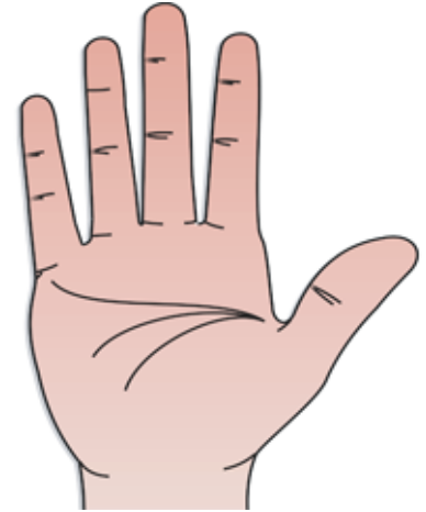
Saturn-Fourth
