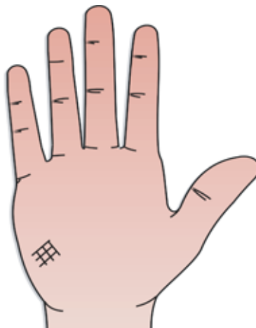
Rahu-Fifth
