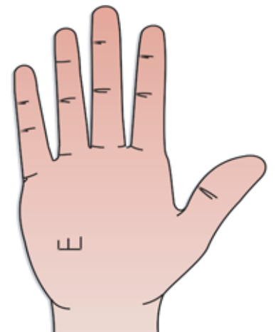
Ketu-Eleventh
