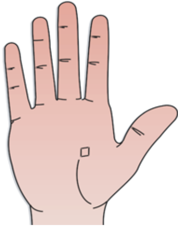
Mars-Third
